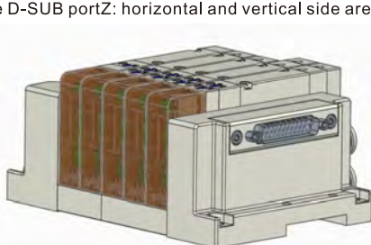
Horizontal plug-in
